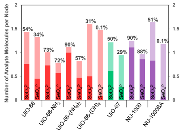
Figure 2. Bar graph illustrating the number of selenate or selenite molecules adsorbed per node in a series of Zr-based MOFs. Light colored bars in the back indicate the maximum possible per node adsorption based on the concentration of the solution (100 ppm Se; 5 mL, pH 7) and the amount of MOF present (10 mg). Dark colored bars indicate the actual per node adsorption calculated using the molecular weight of each MOF. For additional comparison, adsorption per node is given, above each bar, as a percentage of the maximum possible adsorption (i.e., the starting concentration of the solution used).
