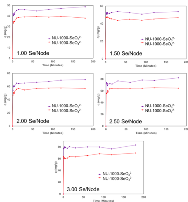
Figure 7. Amount adsorbed ( q ) vs time at various concentrations of selenate and selenite per node of NU-1000.
